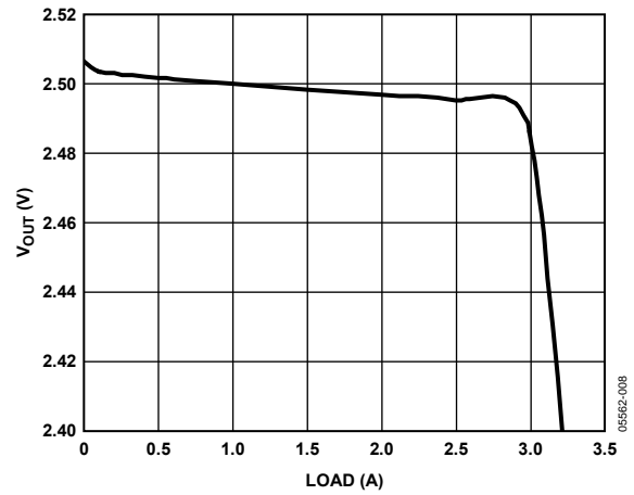
Figure 7. Typical Load Regulation ( V_{IN} = 5\text{ V} ; See Figure 1)
